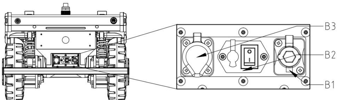
Figure 3 -4 Schematic Diagram of Tail Electrical Position
